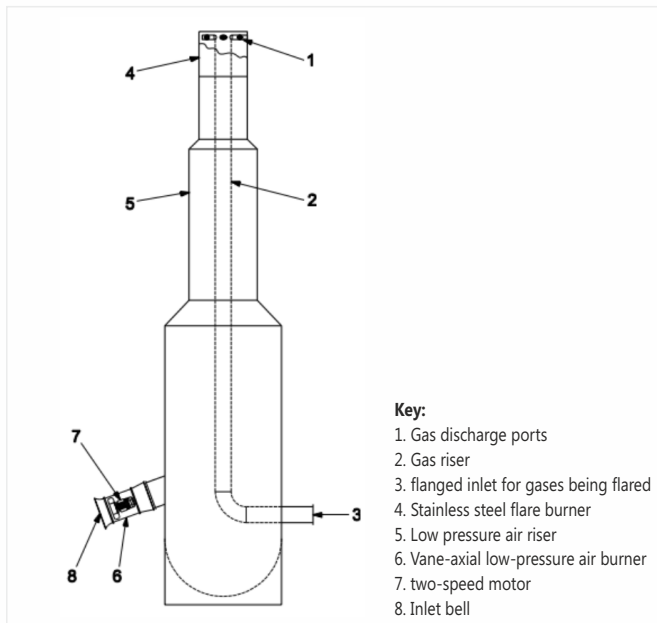
Fig.2. Air-assisted Flare [7]
