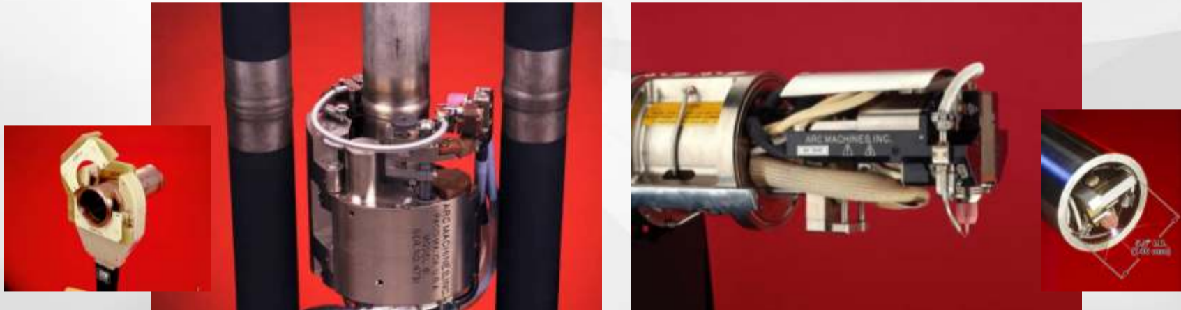
Low Clearance weld head
